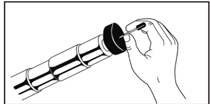
INSERT FASTENER INTO THE MUZZLE END OF THE TOOL WITH THE POINT OUT
