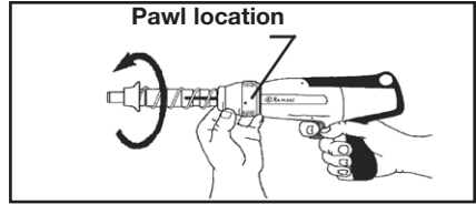
UNSCREW THE BARREL RETENTION COLLAR
